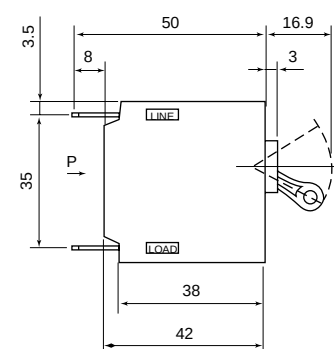
Series trip
